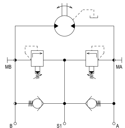
Double pressure relief valve
