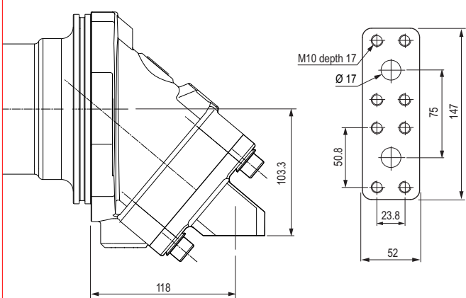
R45 SAE flange ports, bottom 40 degree A and B SAE 3/4" 6000 psi
