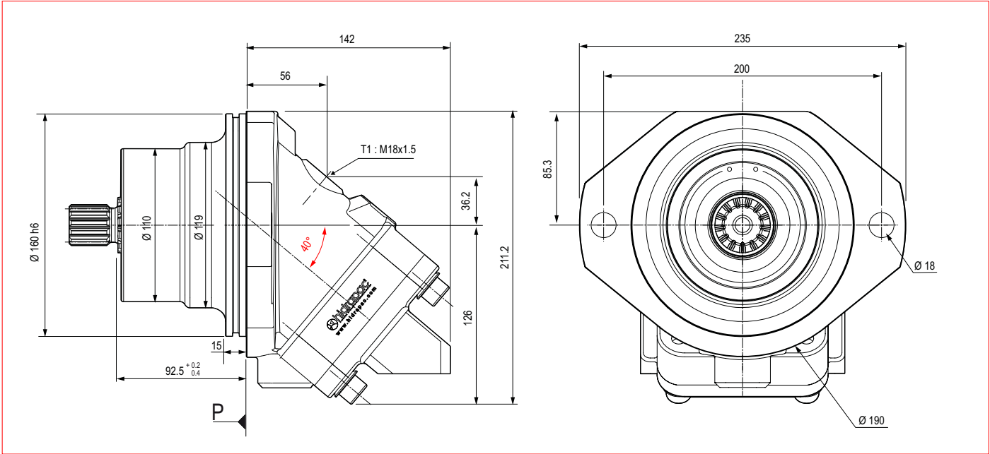
S14 Splined shaft DIN 5480 W 30 x 2 x 30 x 14 x 9 g
