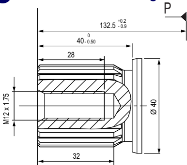
S16 Splined shaft DIN 5480 W 35 x 2 x 30 x 16 x 9 g
